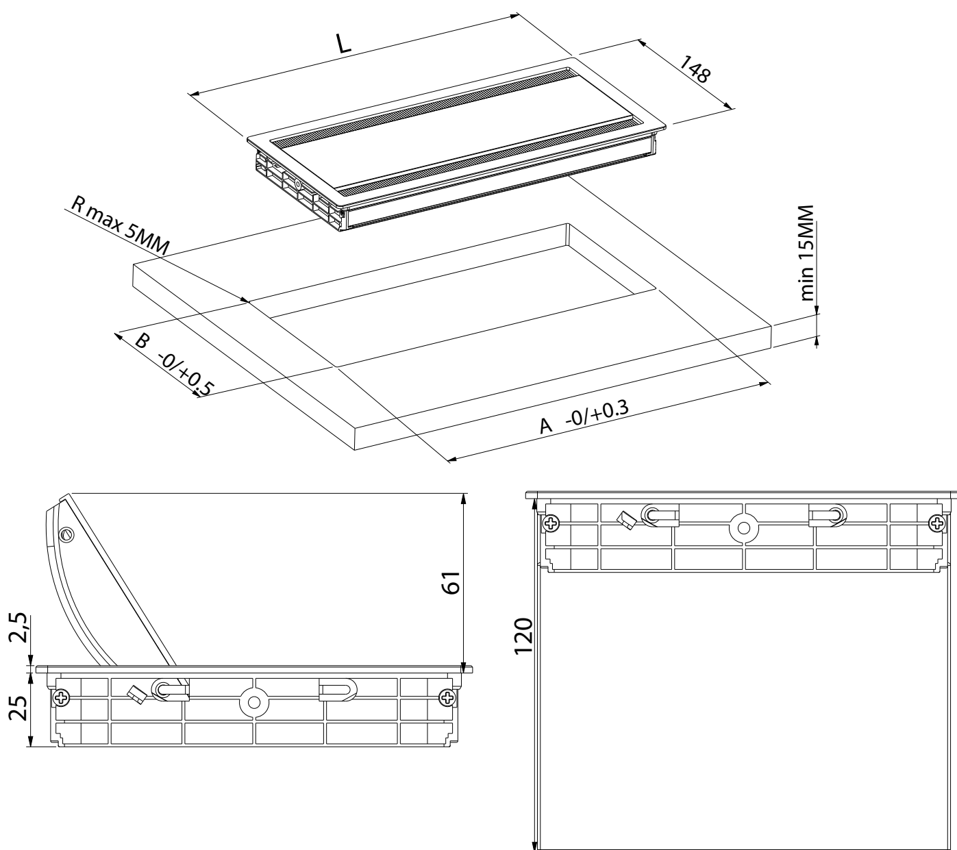
Vasca porta cavi / Cable tray
