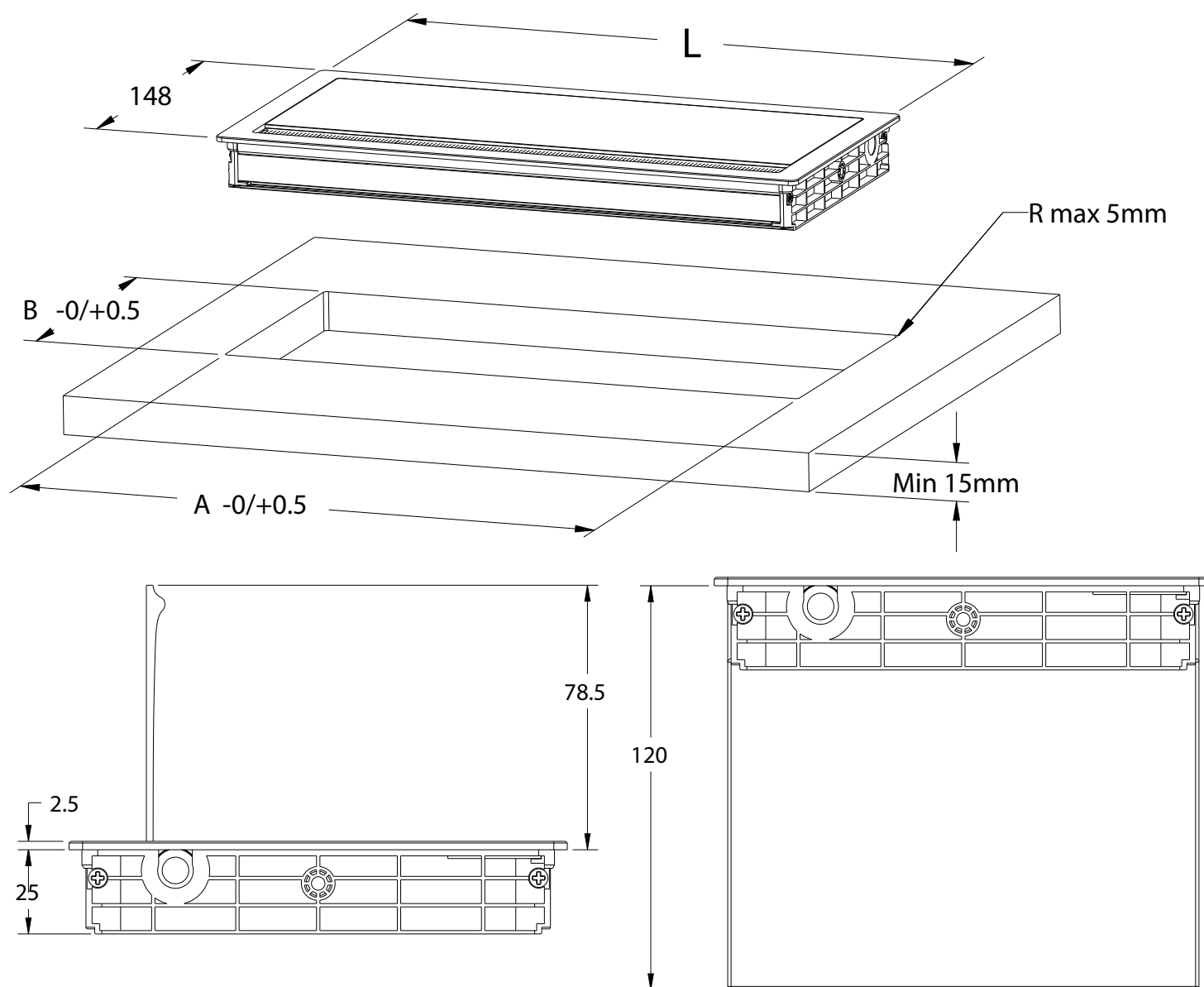
VASCA PORTA CAVI / CABLE TRAY
